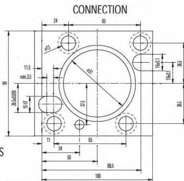
Drill socket
