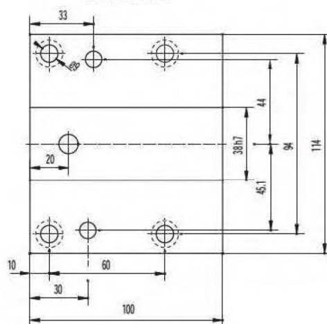
Drill socket
