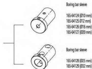
Boring bar sleeve
